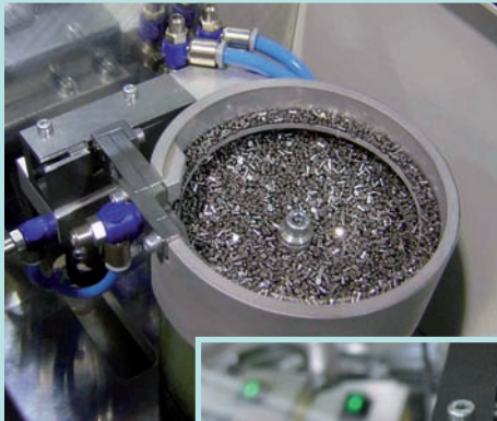
Delivery system ZSE 1000 for pins with 1 mm diameter
