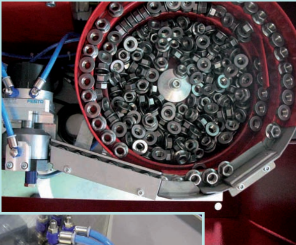
Delivery system with separation for flange nuts
