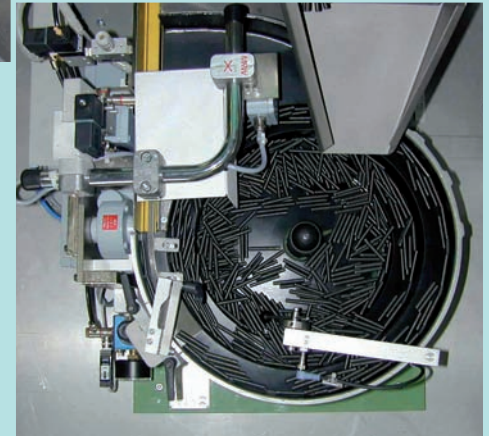
optical sorting with camera
