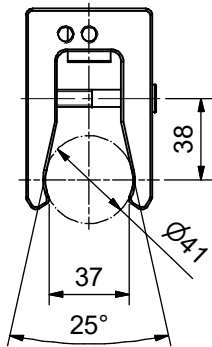
Clamping example
