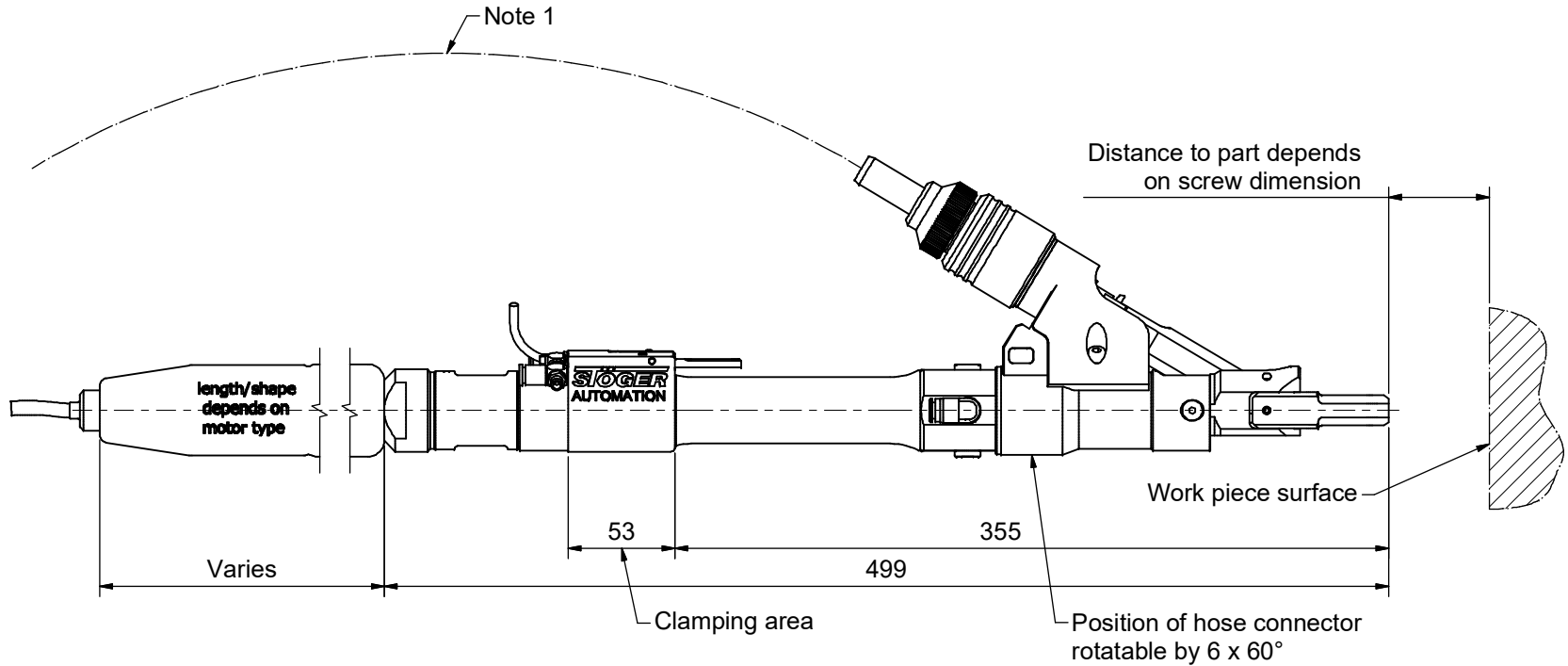
Clamping example
